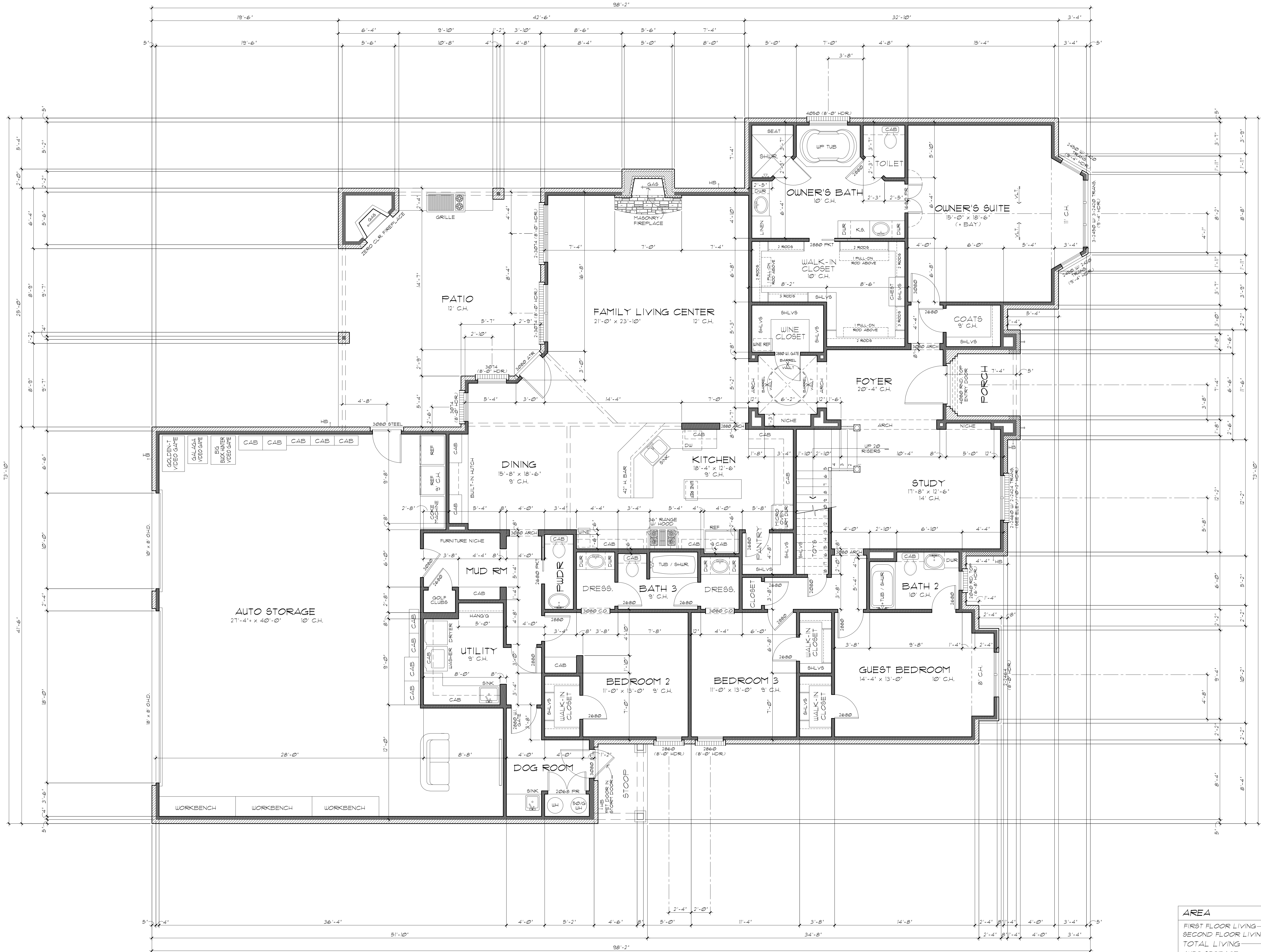
FIRST FLOOR PLAN SCALE: 1/4" = 1'-0"
